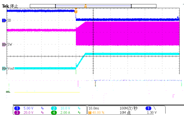
Figure 31. Shutdown remove
