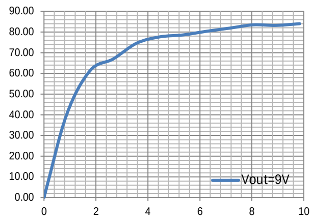
Figure 3. Transfer Efficiency with 10W RX@ Vout=9V
