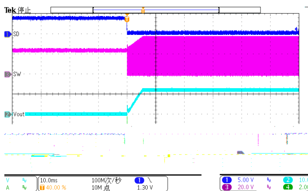
Figure 33. Shutdown remove
