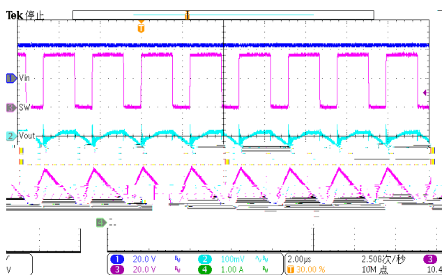
Figure 35. steady-state ( I_{load}=2A )
