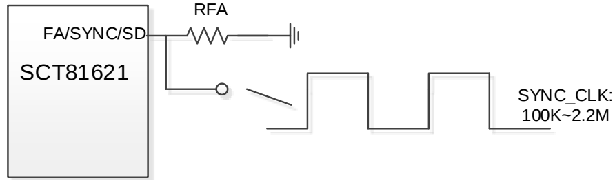
Figure18. Frequency Sync
